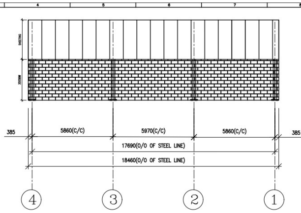
SHEETING ELEVATION ALONG GRID A (ALONG GRID A )
