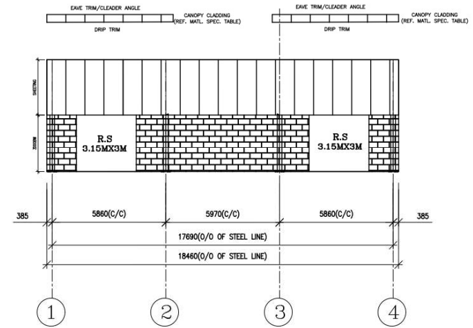
SIDEWALL FRAMING ELEVATION (ALONG GRID C )
