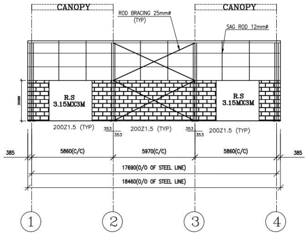
SIDEWALL FRAMING ELEVATION (ALONG GRID C )
