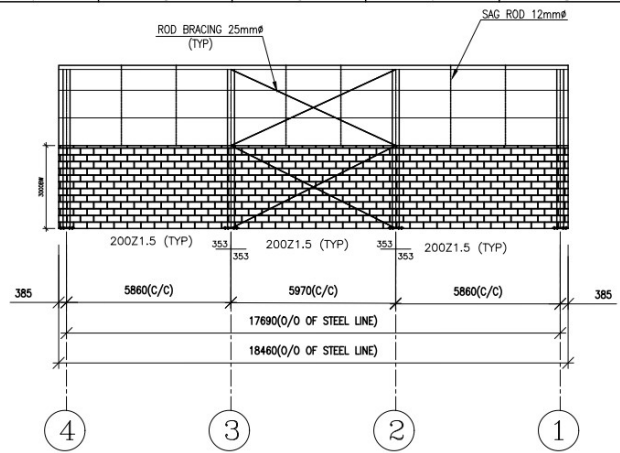
SIDEWALL FRAMING ELEVATION (ALONG GRID A )
